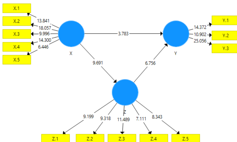
Gambar 4.1. Model PLS
